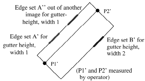
Figure 4: Lopsided saddleback-roof building - edge sets used for the RANSAC algorithm.
