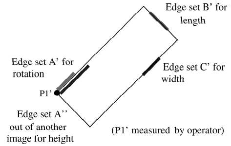
Figure 5: Box - edge sets used for the RANSAC algorithm.
