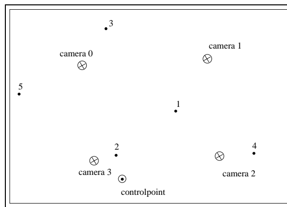
Figure 6: Objectpoints and Camerapositions projected onto the X/Y plane of the object system
