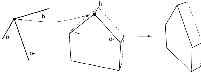
Figure 9: Indexing establishes a link between corner observations (left) and building part primitives (center) resulting in an instantiated building part (right).
