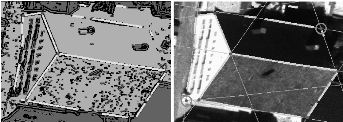
Figure 14: Left: Image features which are successfully matched with the image model of the building hypothesis. Right: 2D corners, predicted by the matched image model depicted by circles and line intersections.
