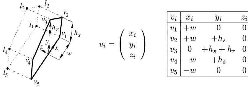
Figure 8: Parameterised description of a hip roof terminal. The table on the right shows the coordinates of the vertices v_1, \dots, v_5 .
