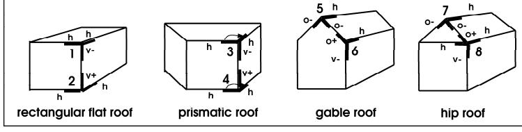
Figure 5: 8 examples of corner classes \omega_c , which are sufficient for describing the building types rectangular flat roof, prismatic roof, gable roof and hip roof, are shown.
