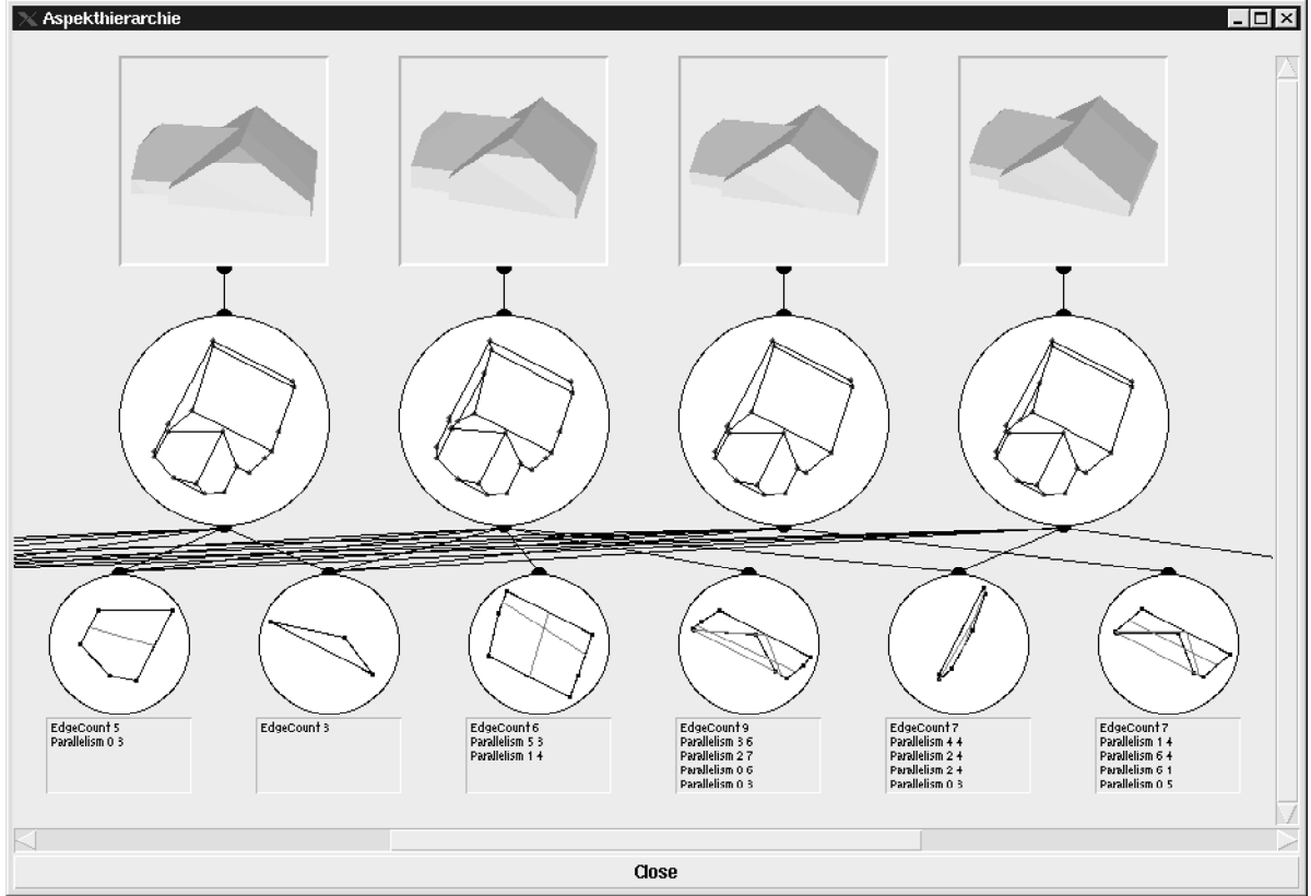
Figure 12: Example of a view hierarchy. For one set of corner reconstructions four different building hypotheses have been generated due to two different indexing results into the library of building parts for the leftmost ridge corner and the free parameter of height (no ground corner was reconstructed).
