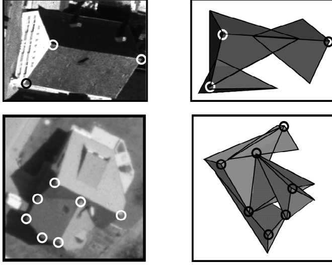
Figure 7: Examples of 3D corner reconstruction. The left column shows the feature aggregates marked in one image. The right column visualizes the reconstructed 3D corners with each corner plane shown as triangle (please note that the corner planes are open ended, the drawn lines solely support the visualization).
