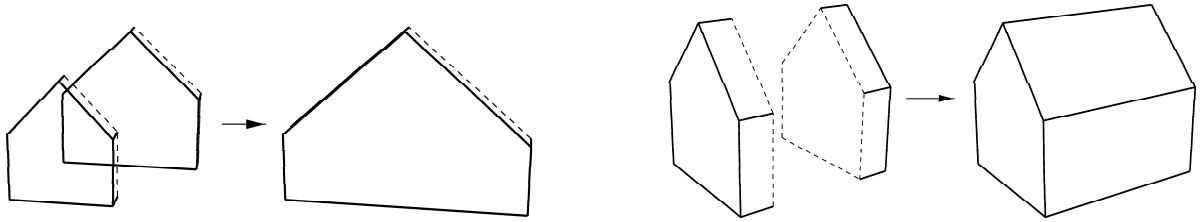
Figure 10: Left: Two saddle roof terminals are merged together. Parameters are adjusted. Right: Two saddle roof terminals are connected together. The resulting building part is closed.
