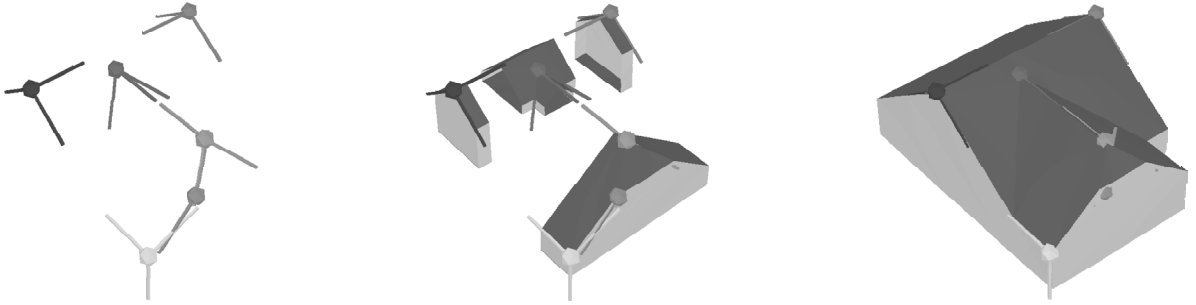
Figure 11: On the left the given corner observations are shown. The figure in the middle shows the best fitting building parts after all indexing steps and some merging steps (building part in the front). These building parts are aggregated in three operations resulting in the building hypothesis shown on the right.
